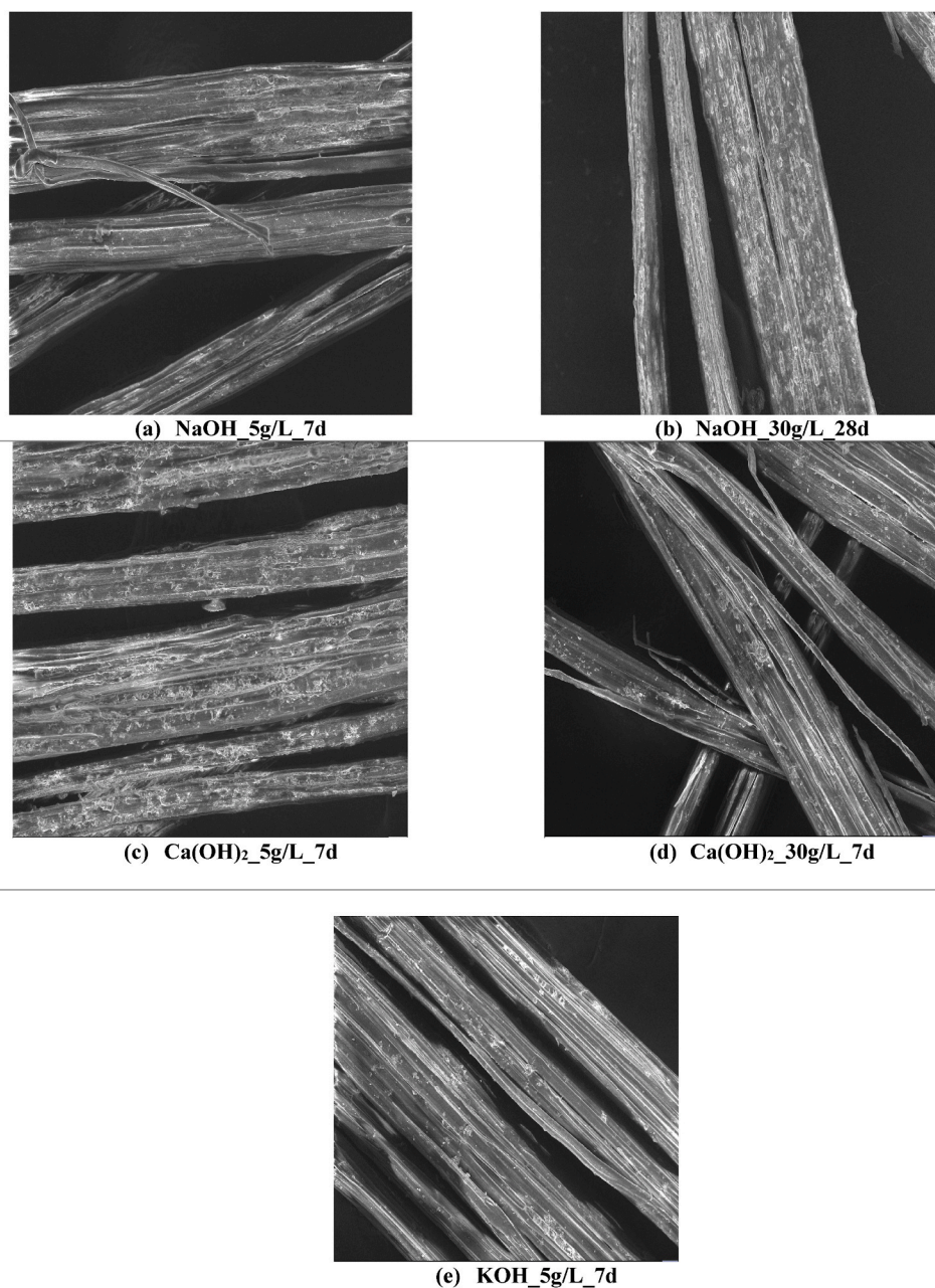
Fig. 8. The SEM outputs of different alkali-treated jute fibres (a,b) NaOH (c,d) Ca(OH) 2 (e) KOH; magnification: 250 X.
