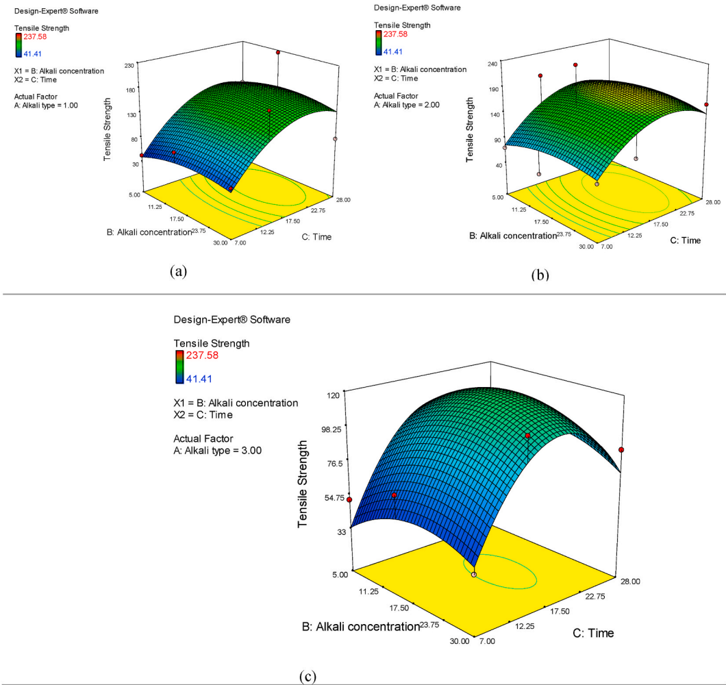
Fig. 14. The graphical result of the optimum condition of tensile strength in (a) alkali type: NaOH, (b) alkali type: KOH, and (c) alkali type: Ca(OH) 2 . applications where maximum tensile strength is a priority, such as in the production of high-strength textiles or composite materials, NaOH or KOH treatment should be considered as the preferred options. Conversely, Ca(OH) 2 treatment may find more relevance in applications where tensile strength is less critical, but other properties like flame resistance or biodegradability are more important. The research aims outlined in this project are closely aligned with sustainability considerations, particularly in the context of jute-based fibres. The initial aim focuses on the preparation of lab-scaled jute-based fiber samples within alkali environments, with a specific emphasis on assessing tensile strength tolerance using the OFAT method. This pursuit is integral to enhancing the durability and performance of jute-based materials, thus contributing to sustainability by potentially extending their lifespan and reducing the need for frequent replacements [73]. Another crucial aspect of the research involves the characterisation of the prepared samples through advanced techniques such as DSC, TGA, and SEM instruments. This characterisation process offers insights into how jute-based fibres behave under varying conditions. Such knowledge is instrumental in optimising their utilisation across diverse applications, potentially resulting in more sustainable end-products. For instance, understanding thermal properties can facilitate the creation of energy-efficient manufacturing processes [74]. The research project also emphasises the optimisation and mathematical modelling of key factors affecting tensile function using the RSM technique. This endeavour has the potential to yield highly efficient processes for jute-based fiber production and application, leading to reduced resource consumption and waste generation. Analysing
