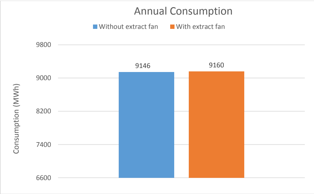
(b) Annual overall energy consumption result
