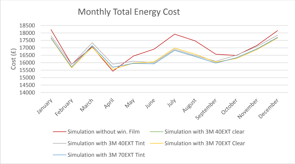
(a) Monthly overall energy cost result
