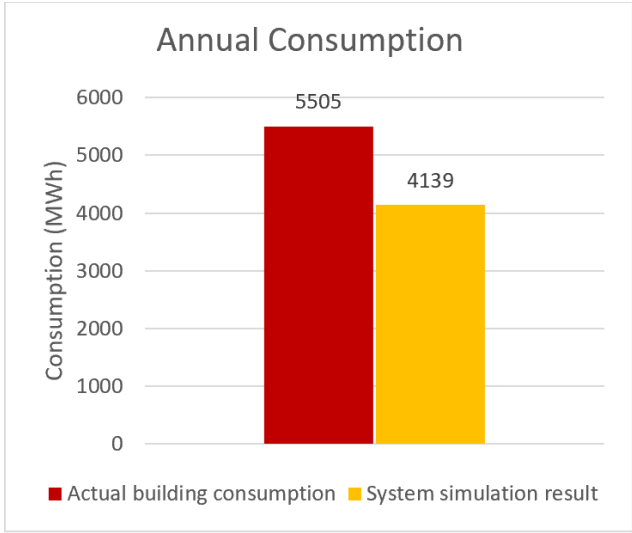
(b) Annual TAS Systems result vs. Actual building consumption
