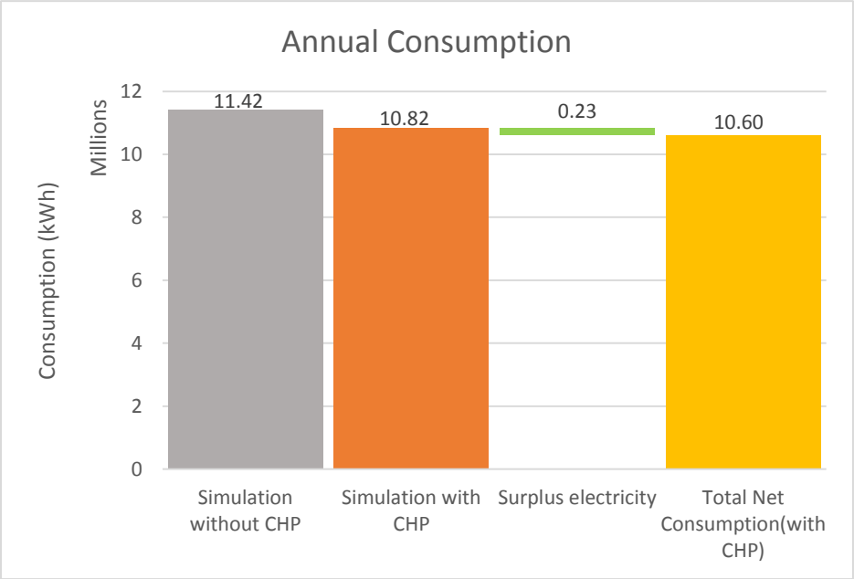
(b) Annual total energy consumption
