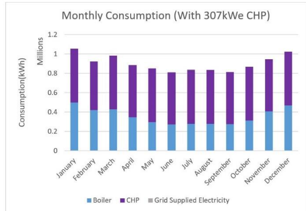
(b) Monthly total energy consumption with CHP
