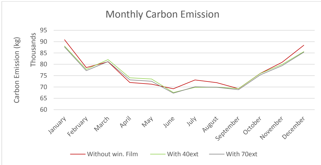
(a) Monthly carbon emission
