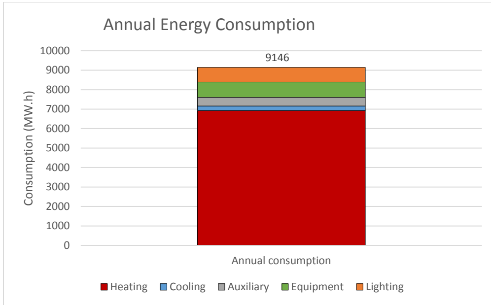
(a) TAS systems simulation result showing annual demand and consumption
