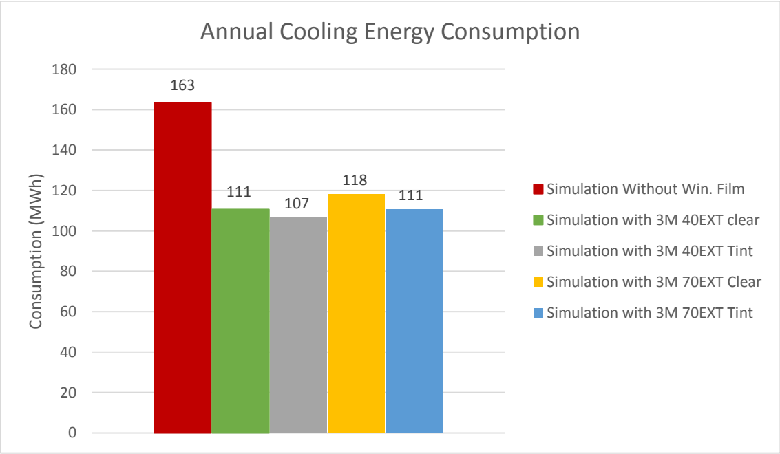
(b) Annual overall cooling energy consumption results
