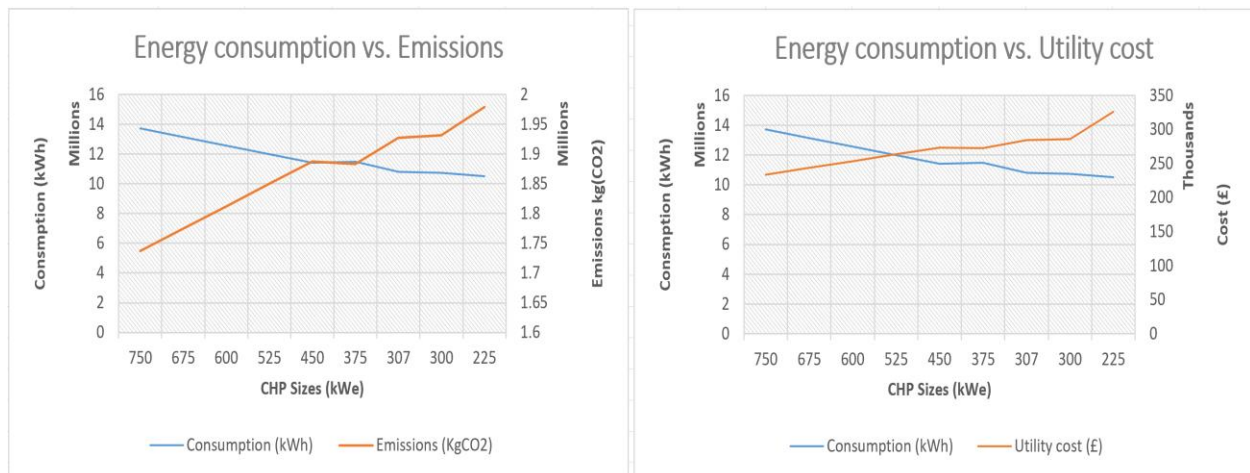
(a) End use energy consumption vs. CO 2 emissions
