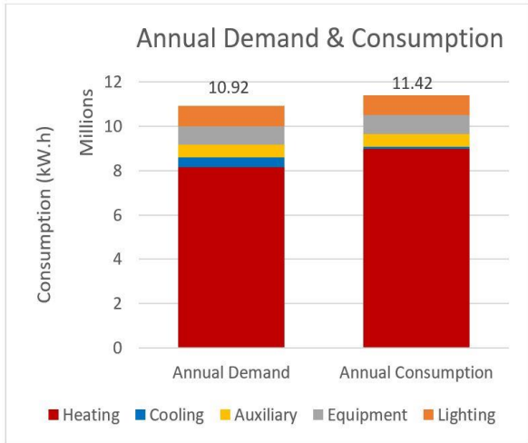
(a) Building model result showing annual demand and consumption
