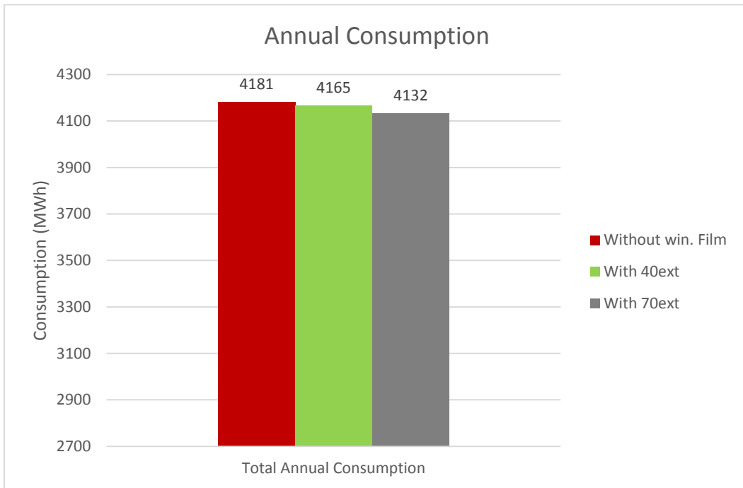
(b) Annual overall energy consumption result
