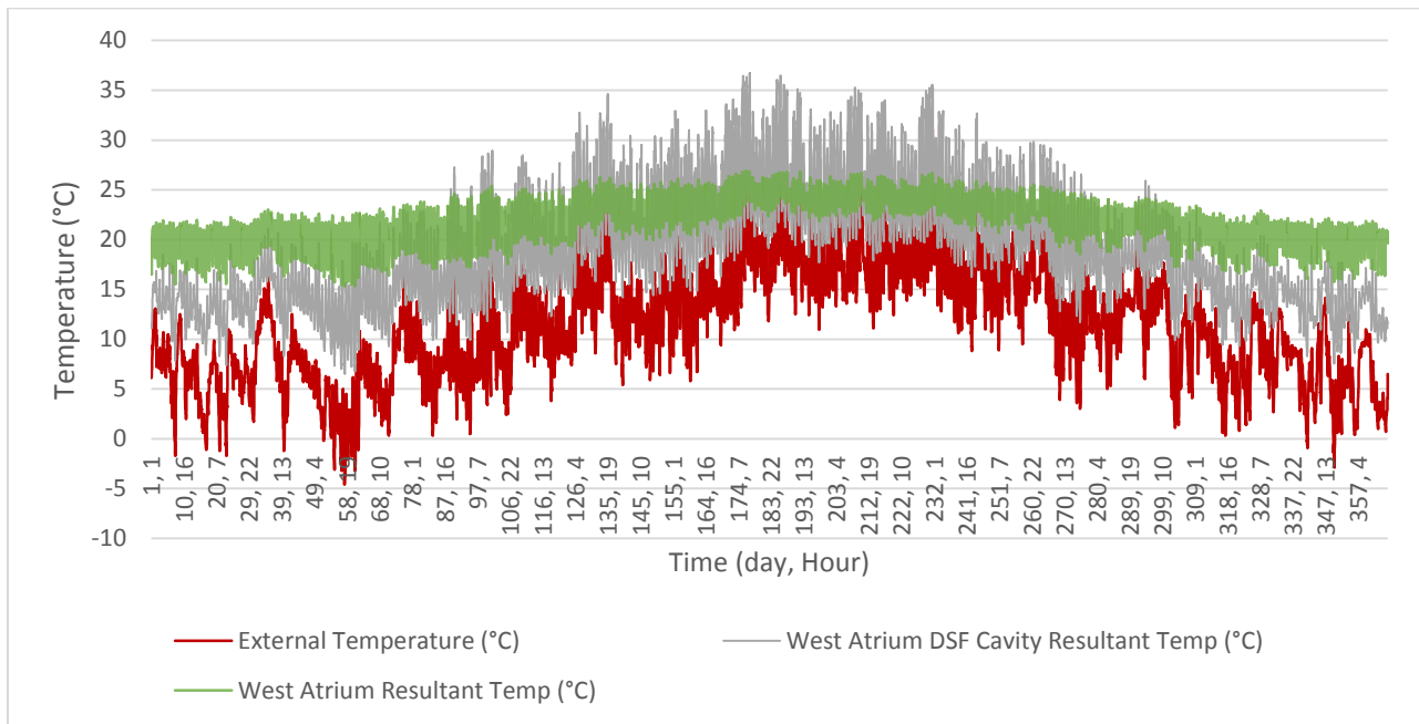
(b) External temperature, West atrium DSF cavity and West atrium resultant temperature vs time (day, hour)
