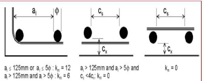
Fig. 4 Reduced effectiveness of transverse reinforcement adapted from fib TG4.5 (2014)
