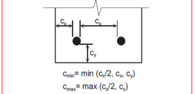
Fig. 3 Definition of concrete cover adapted from fib TG4.5 (2014)
