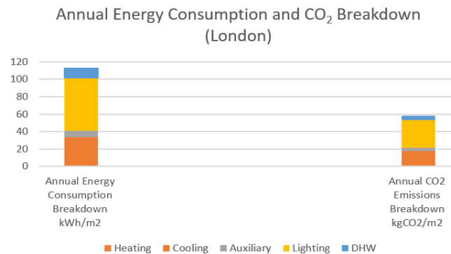
Fig. 6 Annual Energy Consumption and CO 2 breakdown
